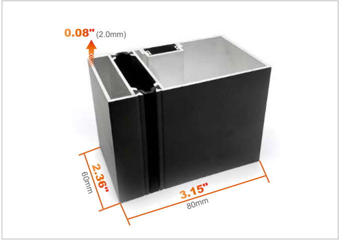
Cross section: Door panel profiles
