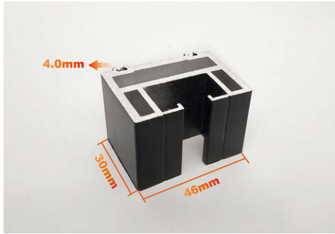
Visible surface: Hinge Stile/Lock Stile
