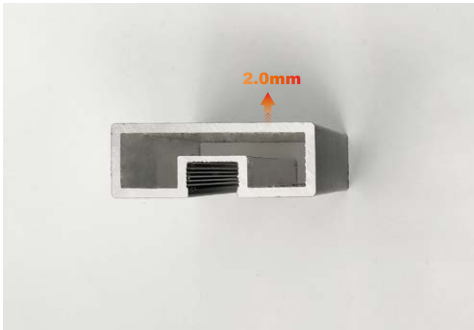
Cross section: Jamb
